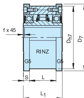
RINZ...G5G5
