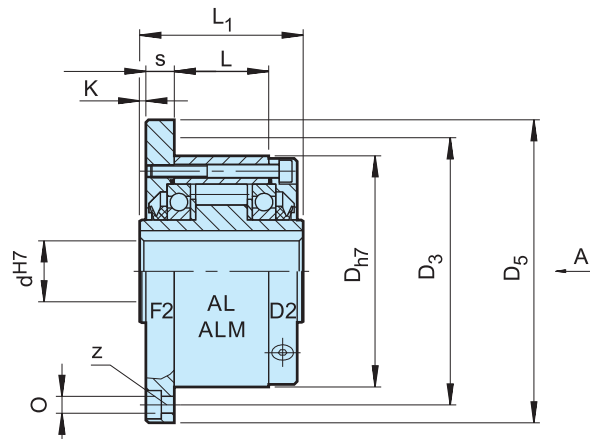
AL..F2D2
